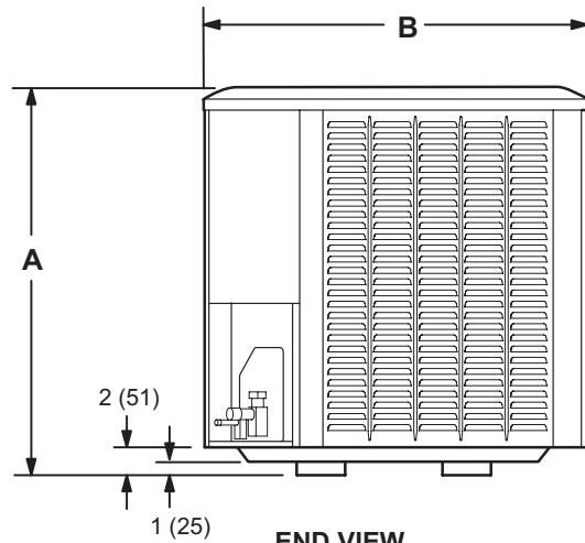
END VIEW
